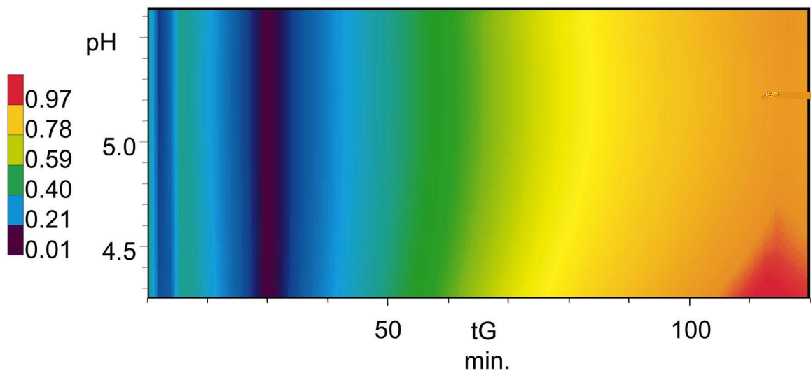
Fig. 8. Plot of the critical resolution against pH and gradient run time ( t_G ) showing the critical resolution. We can see that the pH has no influence on the critical resolution.
